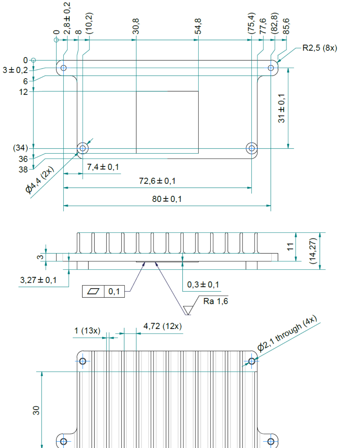
Figure 1-A: Verdin Industrial Heatsink Type 1 Heatsink Dimensions
